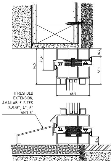
VERTICAL SECTION
