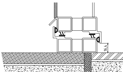
VERTICAL SECTION
