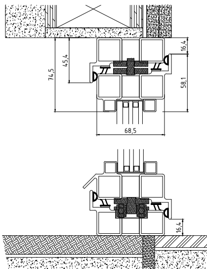
VERTICAL SECTION
