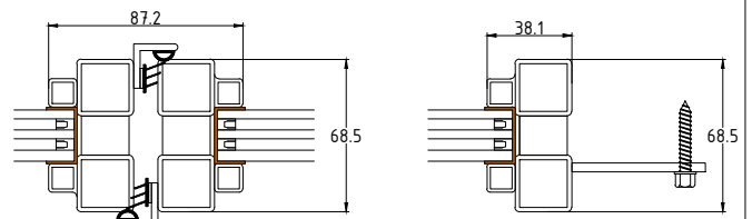
HORIZONTAL SECTION
